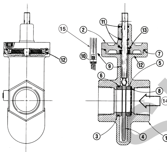
Threaded CP body design shown
