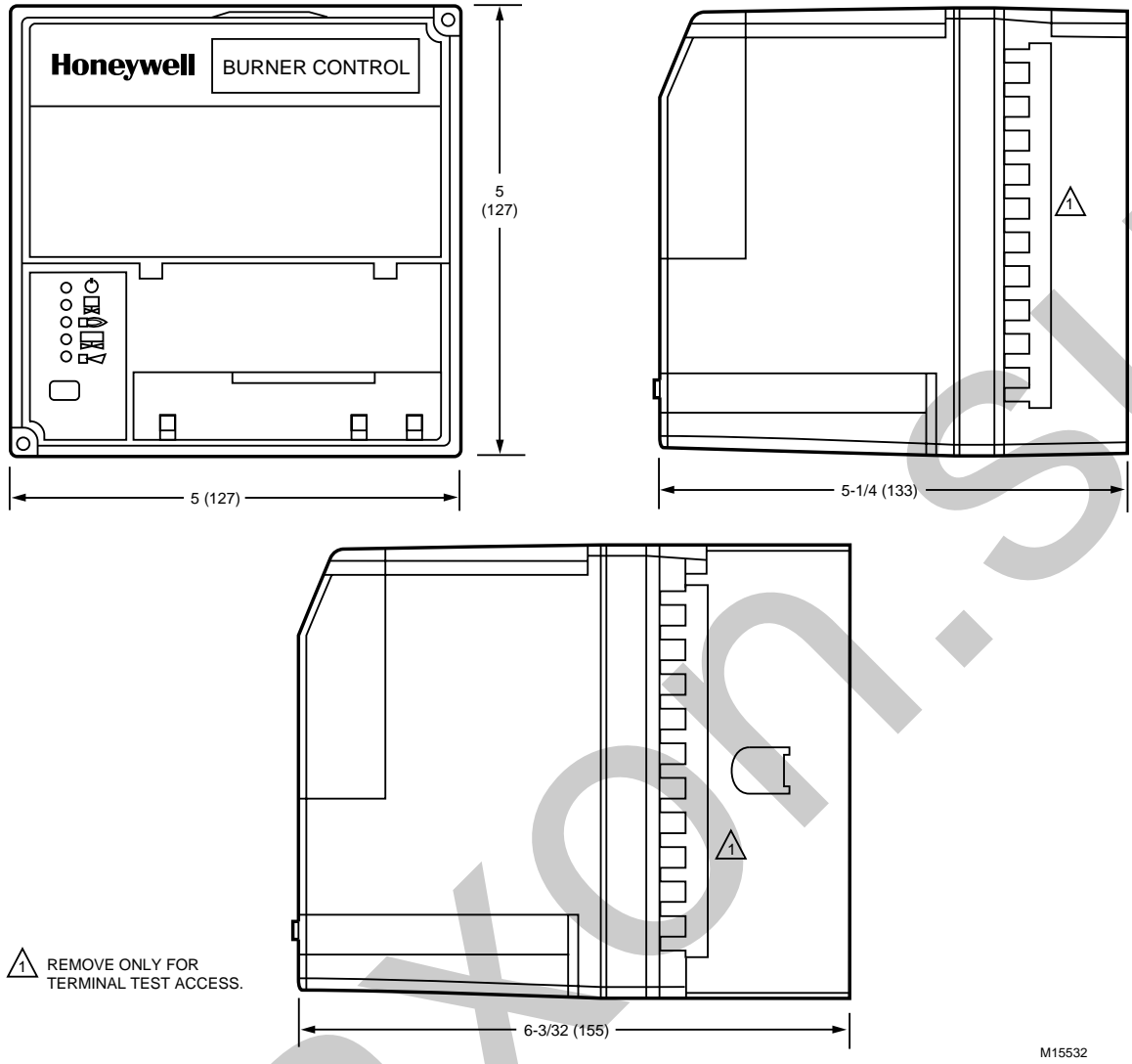
Fig. 2. Mounting dimensions of RM7824 Relay Module and Q7800A and Q7800B Wiring Subbases in in. (mm).
